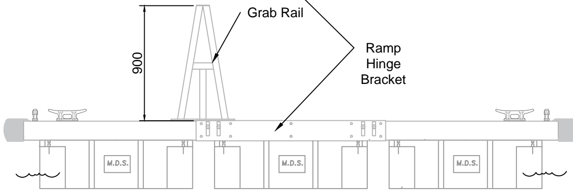
END VIEW
